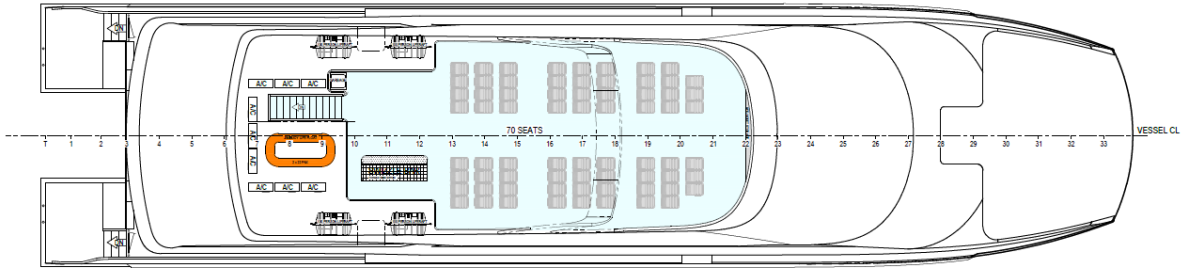
Sun Deck
