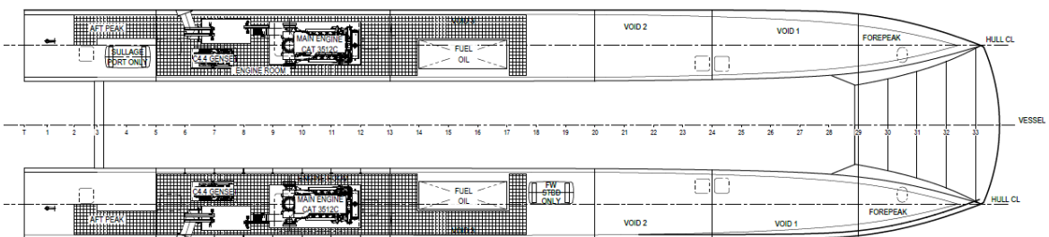
Below Decks
