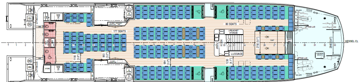
Main Deck
